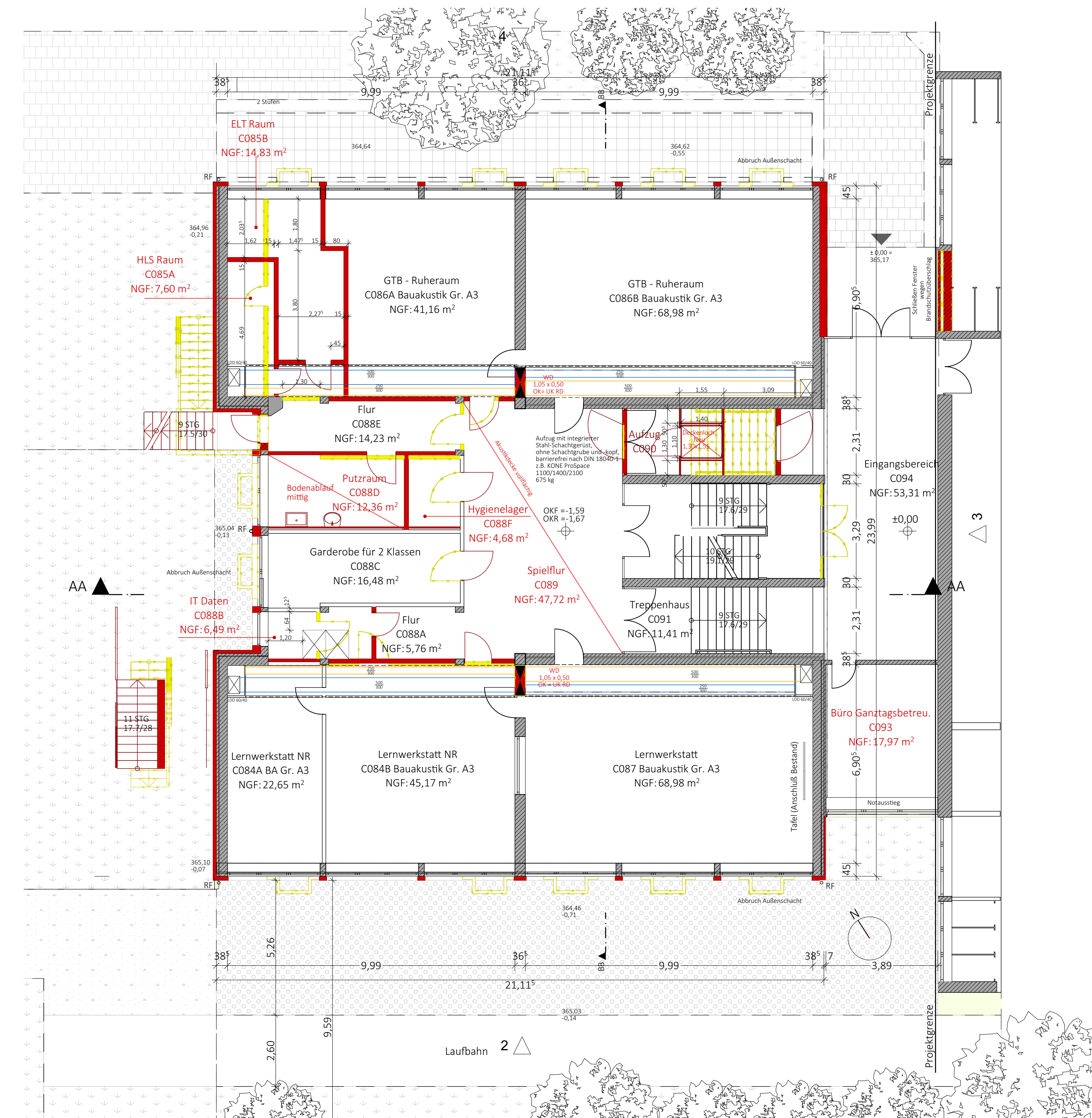
Grundriss Kellergeschoss (Souterrain)
